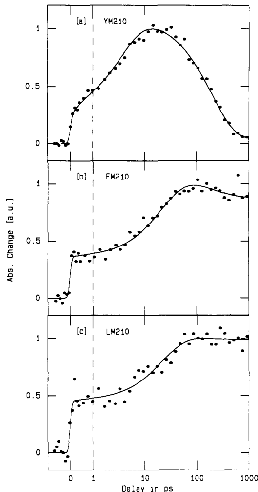
FIGURE 3: Transient absorption data for a probing wavelength of 660 nm using perpendicular polarized pulses: (a) results for wild-type RC (YM210); (b and c) results for mutants FM210 and LM210, respectively. The peak of the absorbance change is \Delta A \approx 0.005 .
